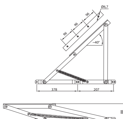
AS 129-1 F_s=360N 0,31 AS 126-1 F_s=550N 0,35 AS 109-1 F_s=630N 0,46 AS 108-1 F_s=900N 0,41 2
