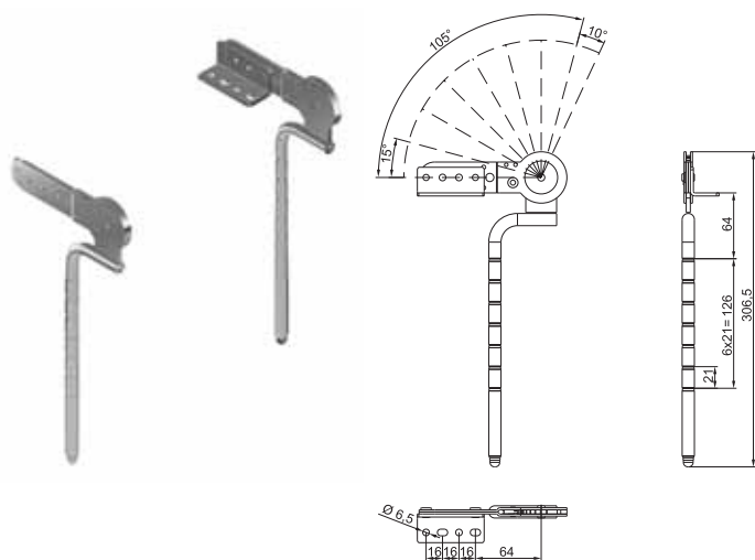
PP 432-B-8 max 105Nm
