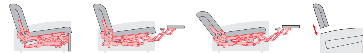
■ Montaż na wsuwki/ Backrest assembled with slide-in joints
